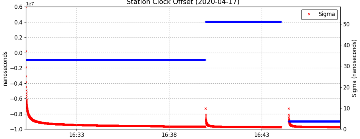
Station Clock Offset (2020-04-17)
