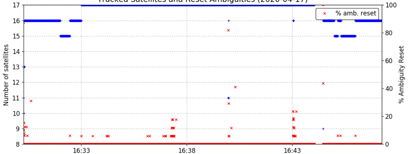
Tracked Satellites and Reset Ambiguities (2020-04-17)
