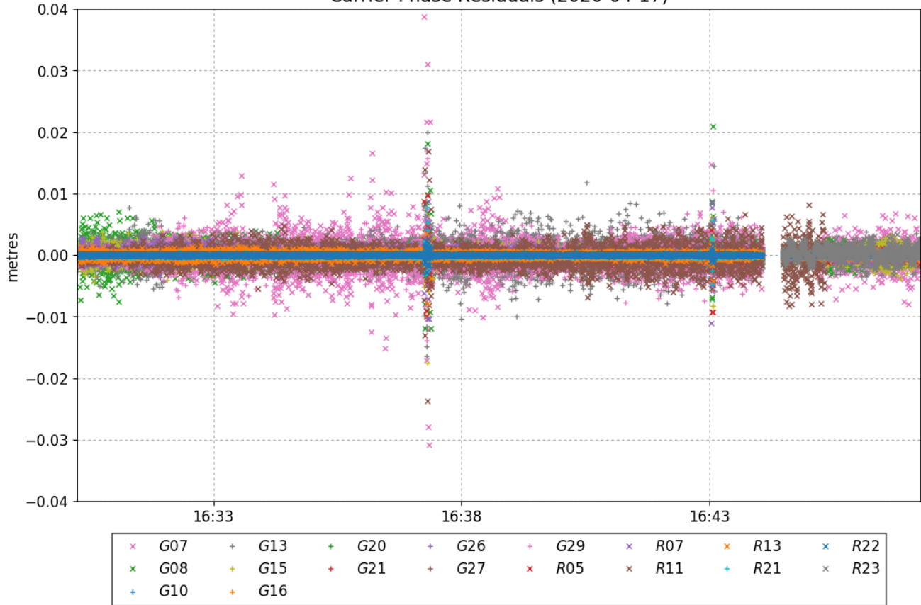
Carrier-Phase Residuals (2020-04-17)
