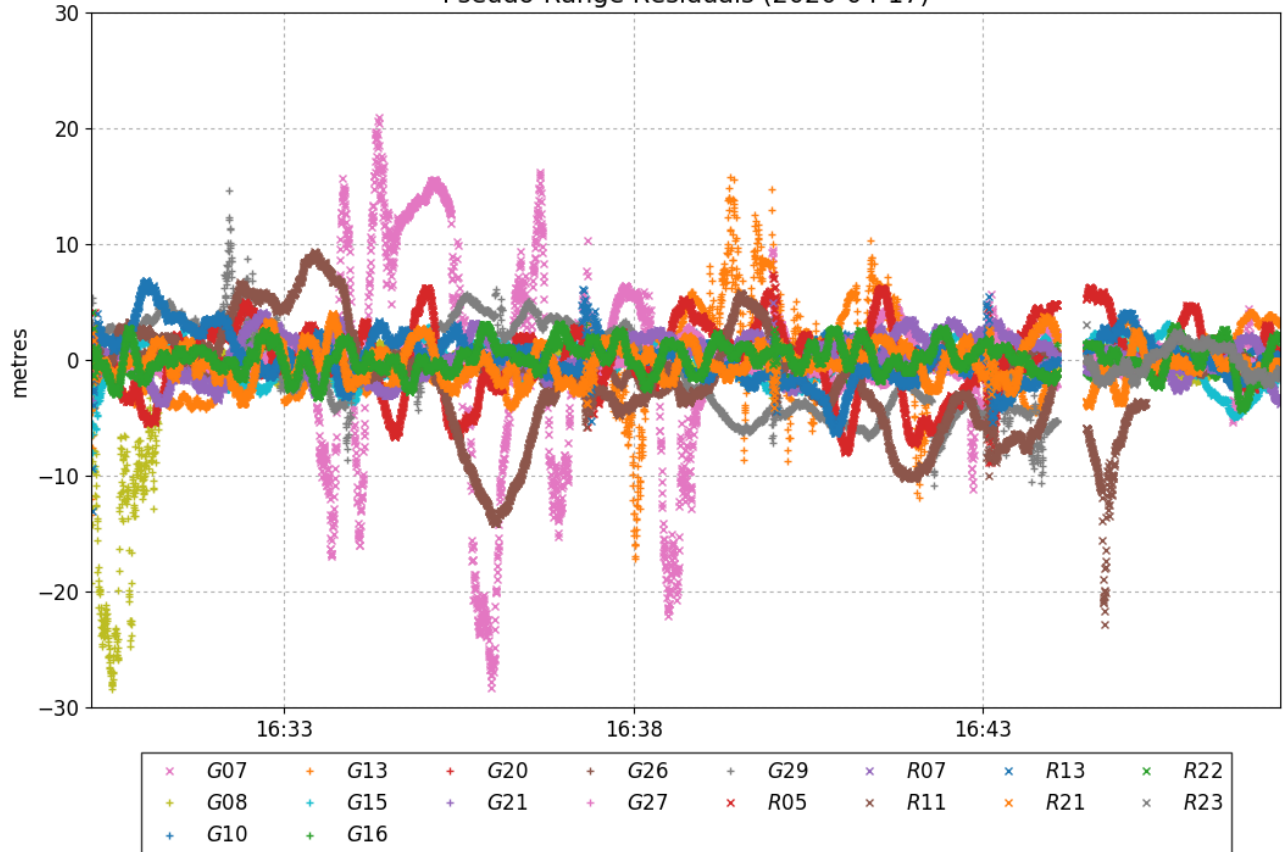
Pseudo-Range Residuals (2020-04-17)
